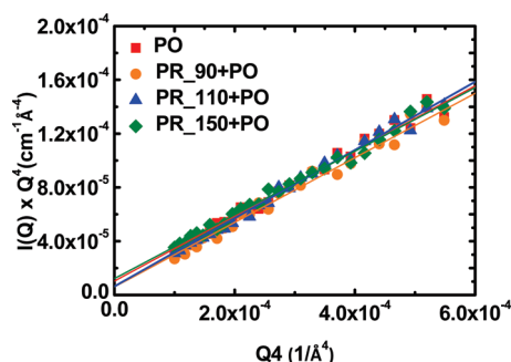
Figure 9. Plot of Q^4 I(Q) vs Q^4 corresponding to Figure S, allowing the determination of K and b values.
